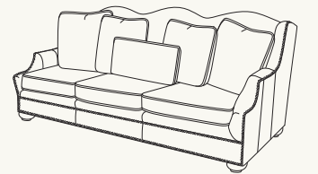
7100-33-01 DRAKE SOFA Overall 79½W x 42½D x 41½H in. Seat 21½H in., Arm 25½H in. Inside 69½W x 28D in. Standard Seat Cushions Spring Down Standard Features Two 24" Throw Pillows, Two 22" Throw Pillows, One 23 x 15" Kidney Pillow, Nail Head Trim Standard Finish Available Only As Shown Shown in married leather, fabrics and finish on pages 34, 35, 36
