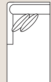
2882 LAF One Arm Chaise 2883 RAF One Arm Chaise Overall: H 37 W 37 D 68 Seating: H 18 W 32 D 48 Seat Height: 19 Arm Height: 25 Pillows: 2 P21
