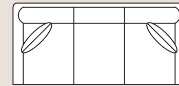
2800 Sofa Overall: H 37 W 84 D 43 Seating: H 18 W 74 D 23 Seat Height: 19 Arm Height: 25 Pillows: 2 P21
