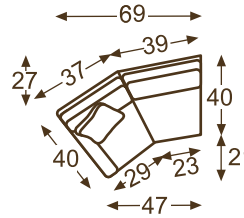
5285-43LF ONE ARM WEDGE SOFA
